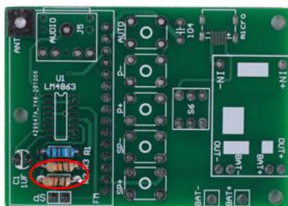
Step 2: Install 2pcs 10Kohm Metal Film Resistor at R2,R3.
