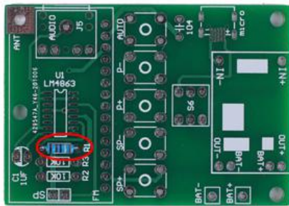
Step 1: Install 1pcs 39Kohm Metal Film Resistor at R1.
